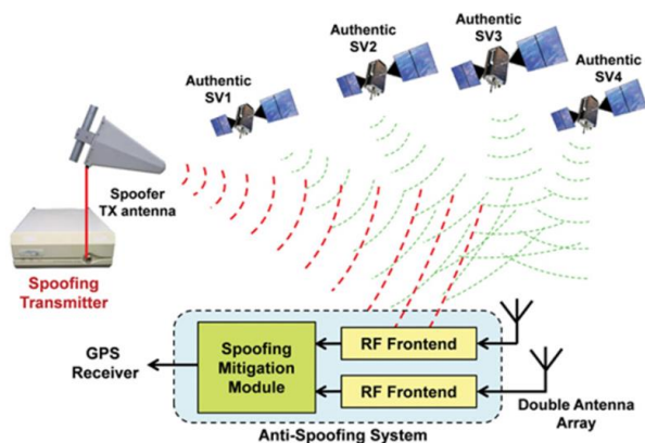
Obr. 2.32: AS systém a GPS. (Zdroj: Daneshmand et al., 2012).
