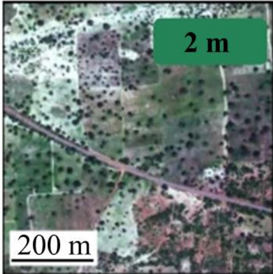
Digital Globe
