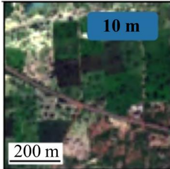
Sentinel-2
