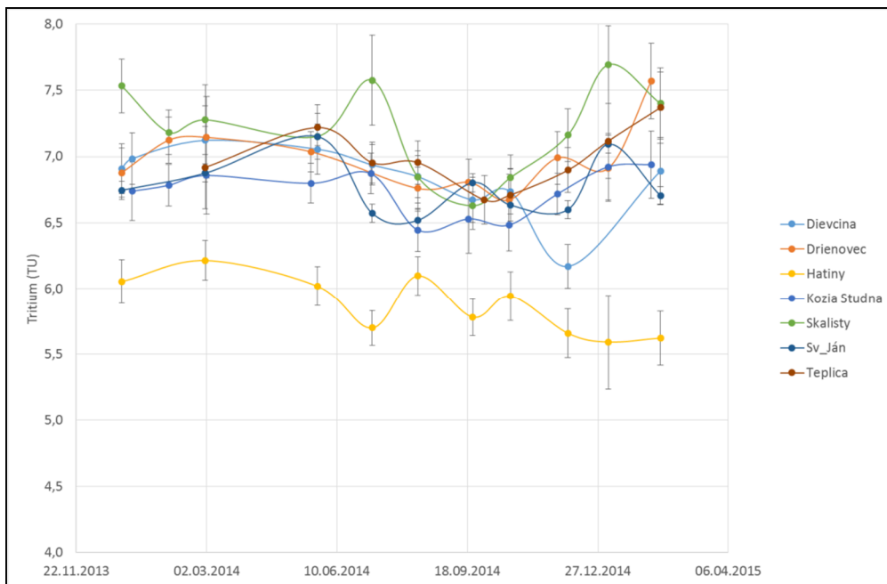
Fig. 7. Tritium concentration at different springs
