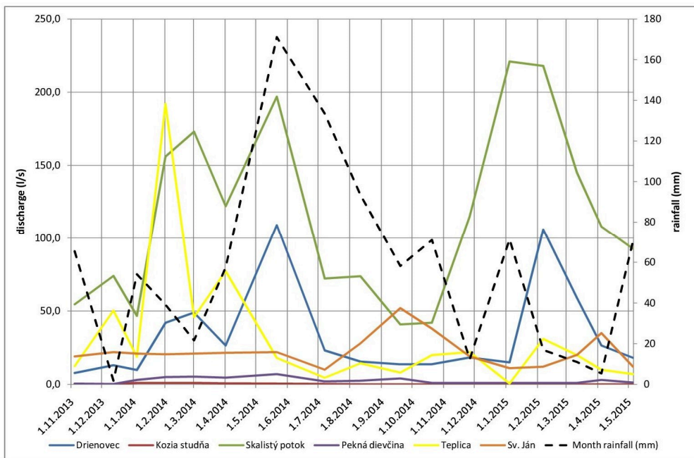
Fig. 5. Rainfall and discharge relationship
