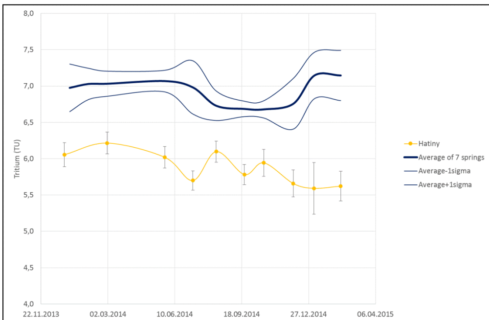
Fig. 8. Average tritium concentrations
