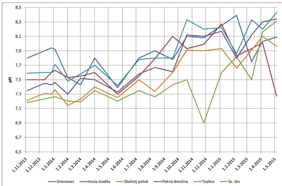
Fig. 4. pH values during the study period
