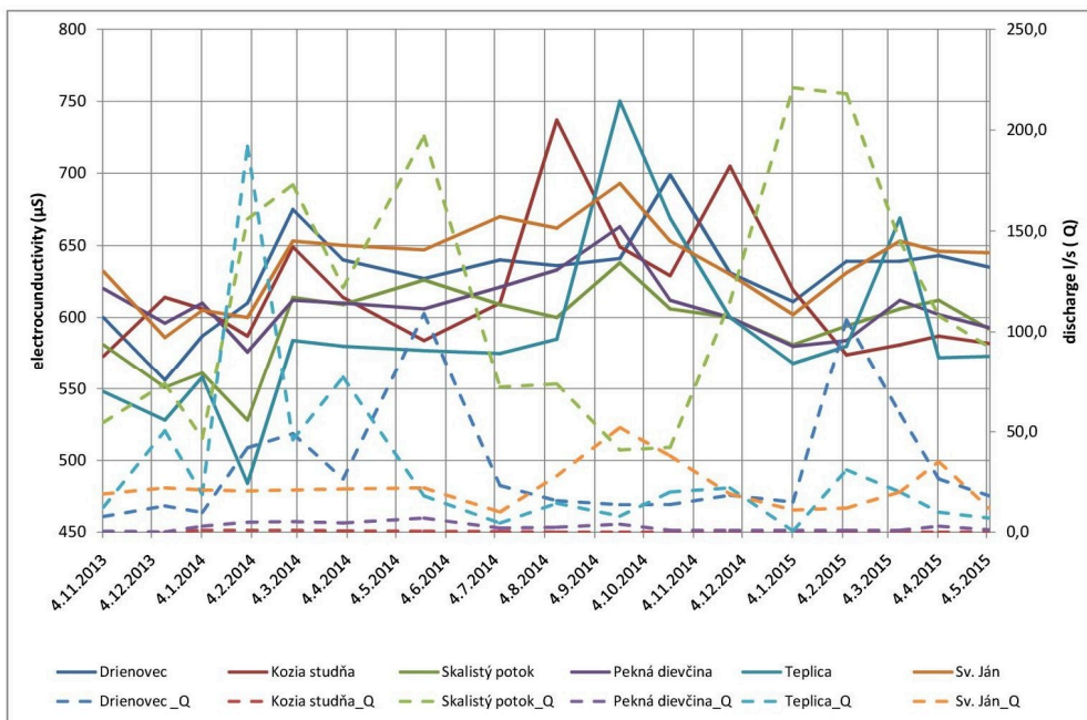
Fig. 3. Electric conductivity and discharge relationship
