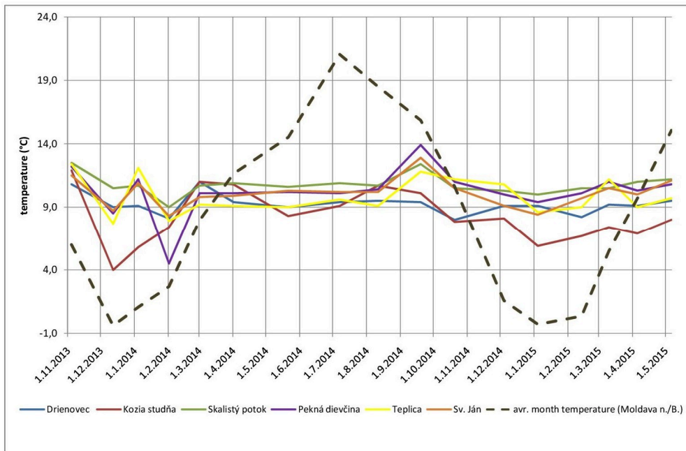
Fig. 2. Relation between water temperature and average month temperature at the springs
